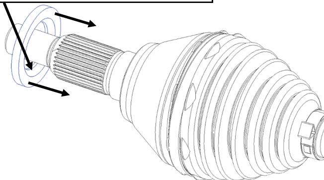
Install CV spacer. Note: Chamfer!
