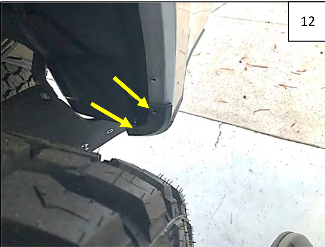
Remove two factory fasteners on rear splash shield.
