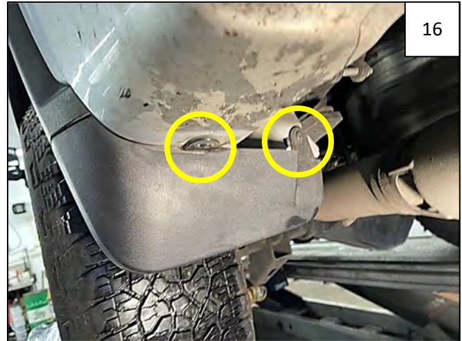
Remove 2 factory screws from underside of splash guard. Remove and discard factory splash guard.
