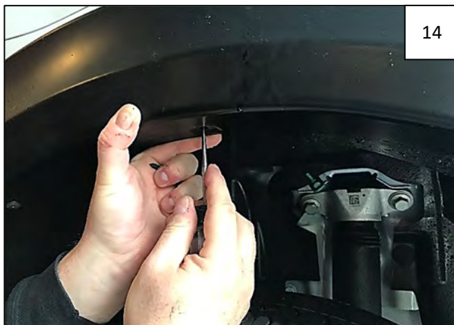
Hold flare firmly on fender. Using a grease pencil, mark 5 hole locations through flare and onto fender lip. This will indicate which plastic fasteners to remove.
