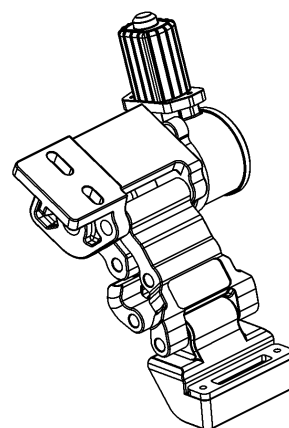
Rear Right Motor x1 Passenger Side
